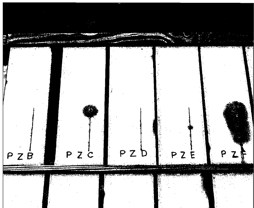
■ Fig. 3 Five replicates showing variable undercutting (three-coat polyamide at approximately 4 years)
