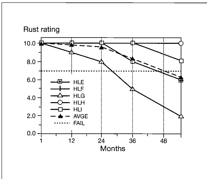
■ Fig. 2 Alkyd in marine, 5 replicates; average of 5 panels
