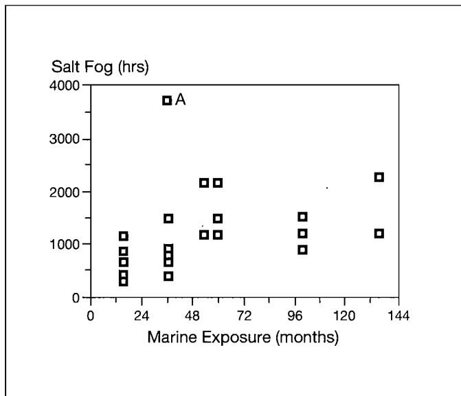
■ Fig. 4 PACE, Branch A, lead- and chromate-free oil/alkyd. Each point corresponds to a specific coating system. (E.g., for coating A, rust failure in salt fog occurred after 3,700 hours, and rust failure at marine exposure occurred after 36 months.)
