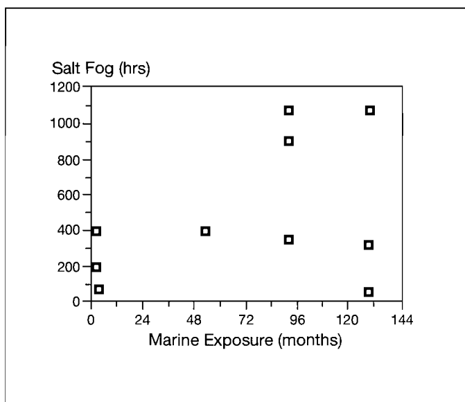
■ Fig. 5 PACE, Branch C, acrylic over SSPC-SP 2. Each point corresponds to a specific coating system.
