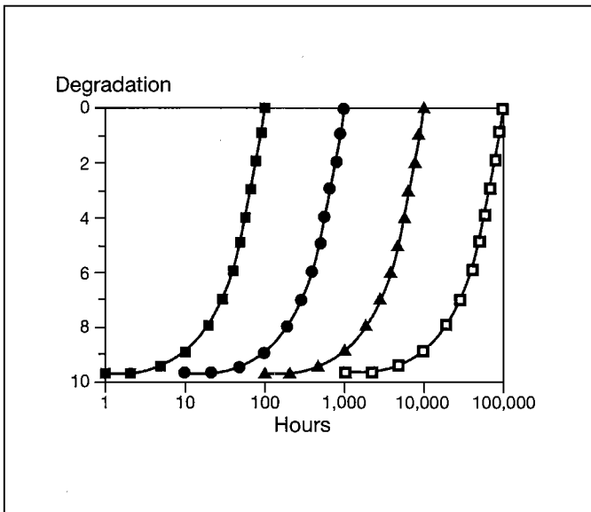
■ Fig. 1 Typical time frames for degradation □ Typical degradation rate based on rusting and undercutting in exterior ▲ Typical degradation rate based on rusting and undercutting in accelerated testing (e.g., salt fog) or early indicator (e.g., electrochemical response) in exterior ● Typical degradation rate based on early indicator in accelerated test ■ Degradation rate for new experimental test procedure (sought in future) Note: 1 month = 30 days = 720 hours 1 year = 8,760 hours
