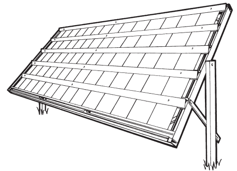
Outdoor testing rack with painted panels.
