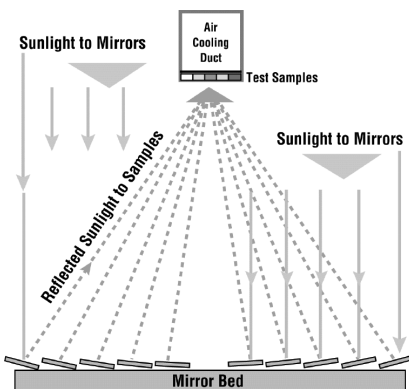
A series of ten mirrors reflect sunlight onto test specimens.
